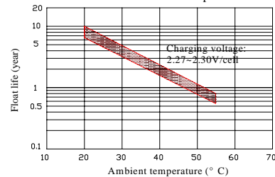
Float service life V'S temperature
